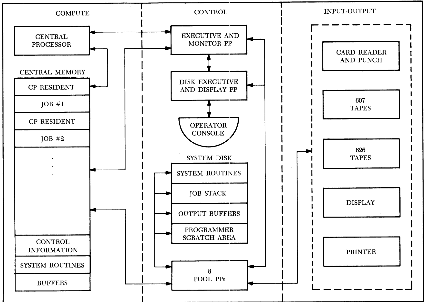
Figure 3. SIPROS COMMUNICATION FLOW
